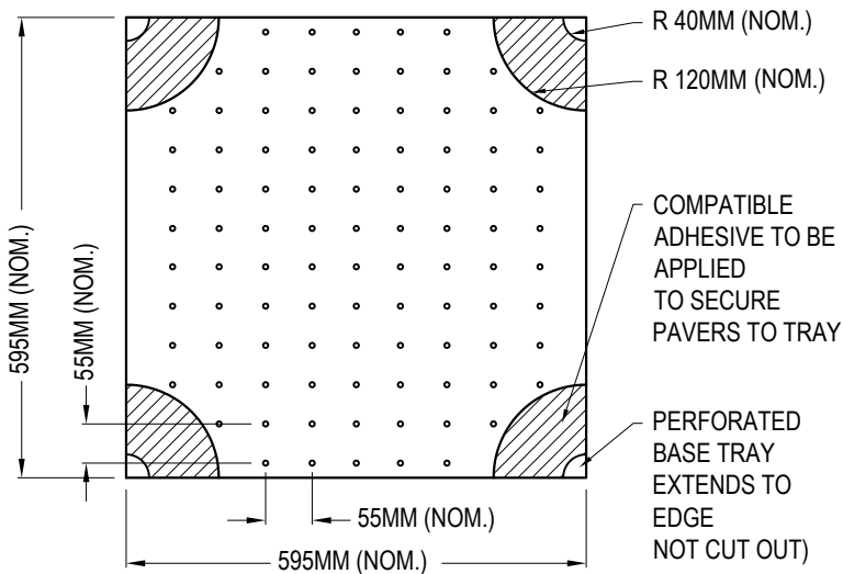
PLAN VIEW RHINO STEEL TRAY
