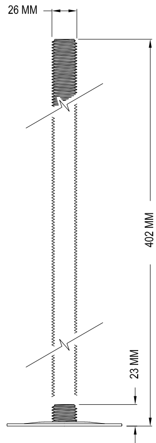
SIDE VIEW BASE
