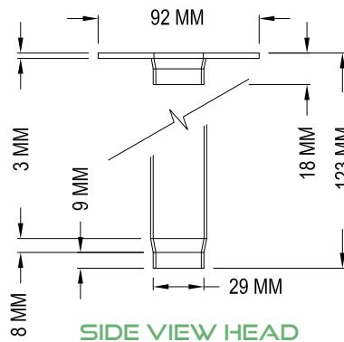
SIDE VIEW HEAD
