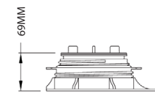
ELEVATION VIEW RHN-SL0-B (MAX. HEIGHT)
