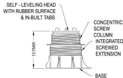
ELEVATION VIEW RHN-SL0-C (MAX. HEIGHT)
