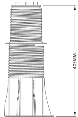
ELEVATION VIEW RHN-SL0-D (MAX. HEIGHT)
