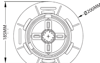
PLAN VIEW RHN-SL0-C
