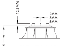
ELEVATION VIEW RHN-SL0-C (MIN. HEIGHT)
