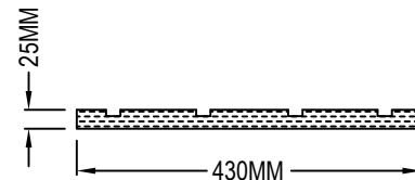
DETAIL VIEW POLYURETHANE FOAM SHEET
