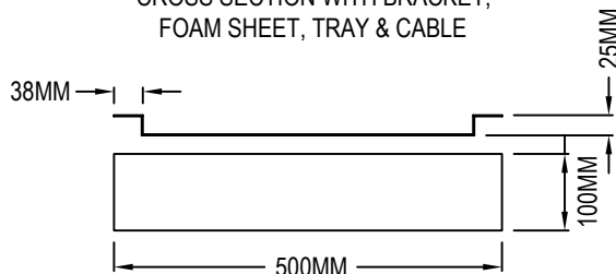
DETAIL VIEW ALUMINUM SUPPORT BRACKET
